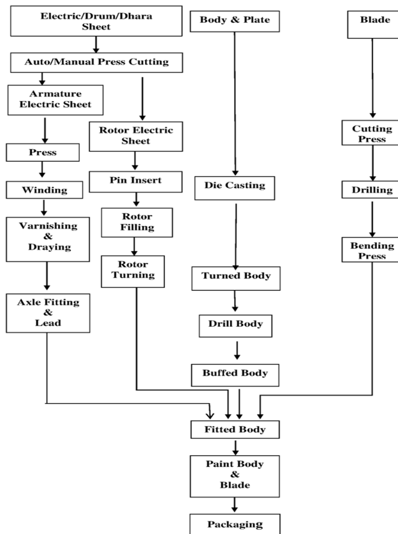
Exhibit 3: Process Flow Chart
