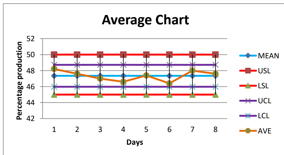
Exhibit 5: SPC Results Before Implementing Obeya
