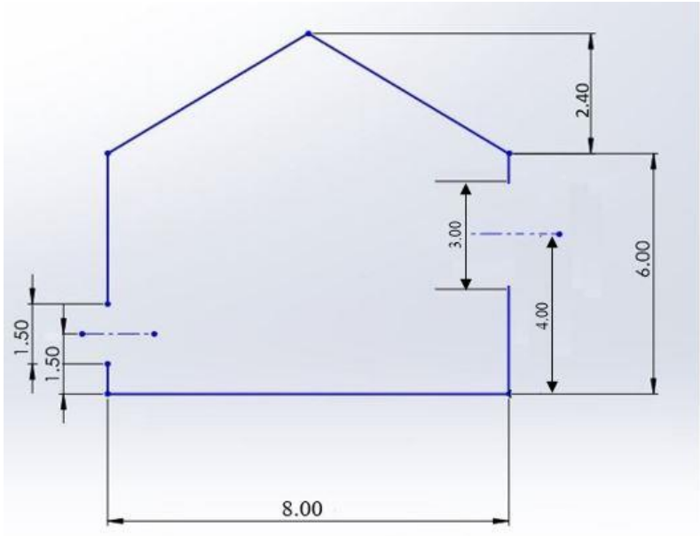
Fig 4.5: Cross Sectional view of Configuration D
