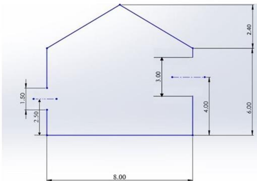
Fig 4.3a: Cross Sectional view of Configuration B1
