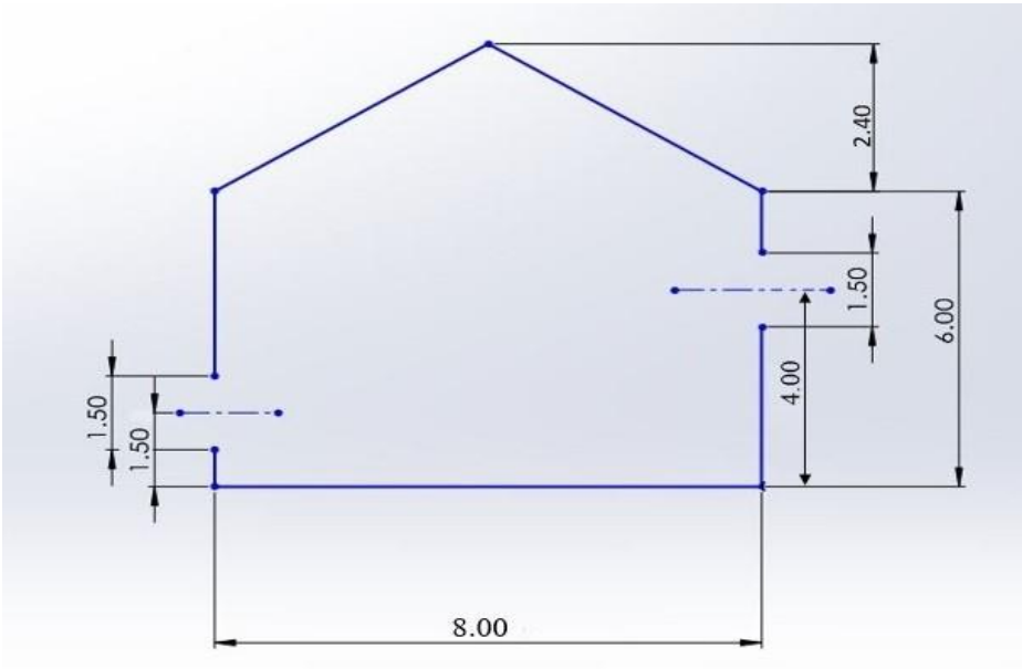
Fig 4.5: Cross Sectional view of Configuration D
