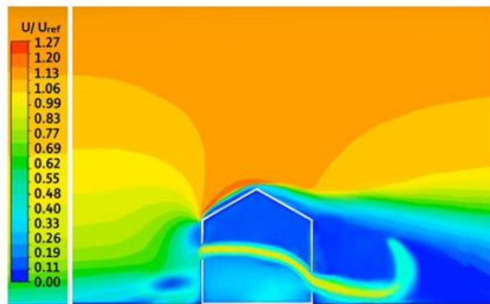
Fig 4.10: Velocity contour for configuration C with wall Porosity 10%.
