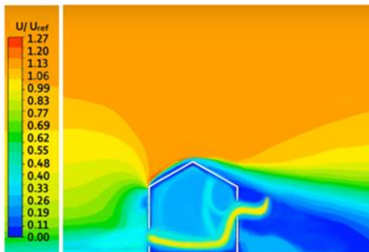
Fig 4.12: Velocity contour for configuration D with wall Porosity 10%.
