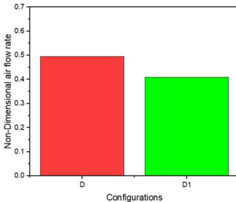
Fig 4.17: Comparison of non-dimensional air flow rate for configuration D and D1
