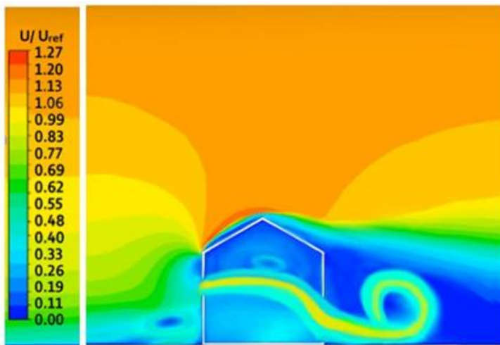
Fig 4.11: Velocity contour for configuration C1 with wall Porosity 10%.
