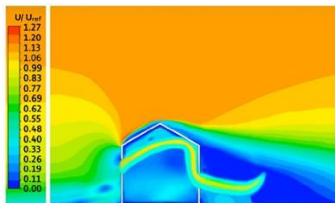
Fig 4.6: Velocity contour for configuration A with wall Porosity 10%.
