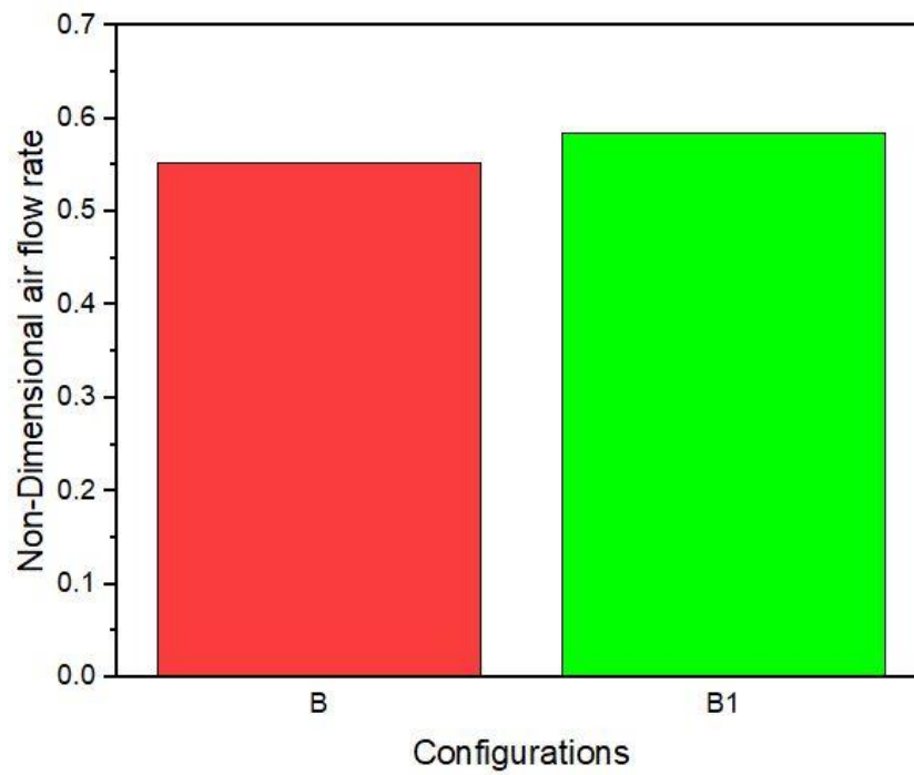
Fig 4.15: Comparison of non-dimensional air flow rate for configuration B and B1
