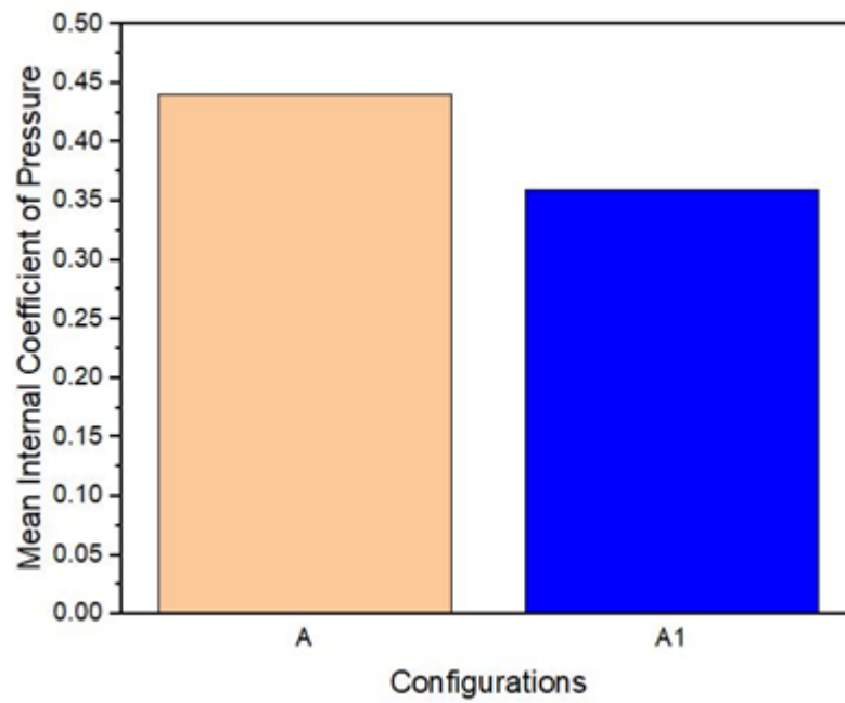
Fig 4.18: Comparison of mean internal coefficient of pressure for configuration A and A1
