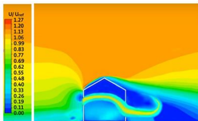
Fig 4.7: Velocity contour for configuration A1 with wall Porosity 10%.
