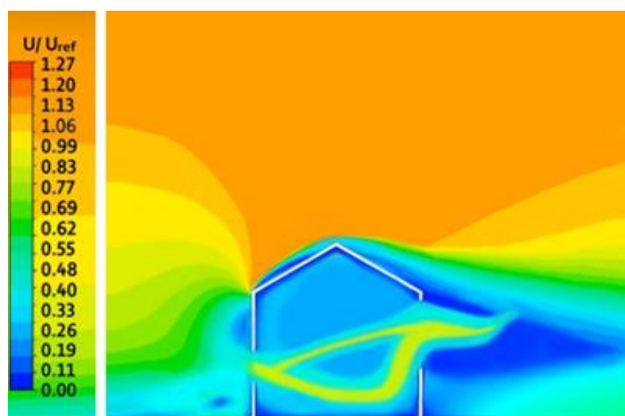
Fig 4.9: Velocity contour for configuration B1 with wall Porosity 10%.
