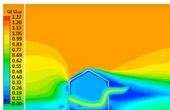
Fig 4.8: Velocity contour for configuration B with wall Porosity 10%.
