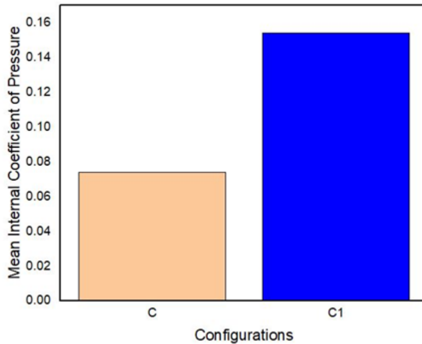
Fig 4.20: Comparison of mean internal coefficient of pressure for configuration C and C1
