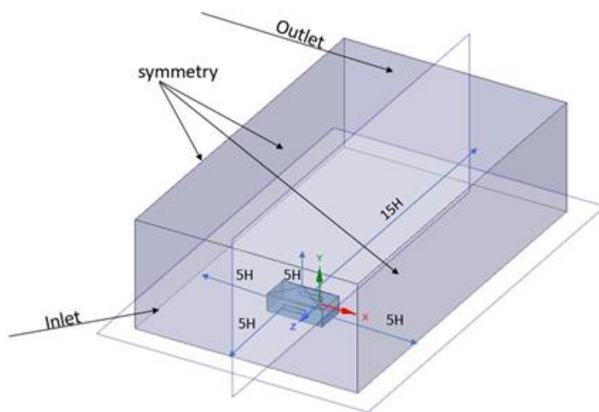
Fig 3.2: Three-dimensional view of computational domain
