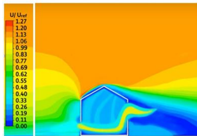
Fig 4.13: Velocity contour for configuration D1 with wall Porosity 10%.
