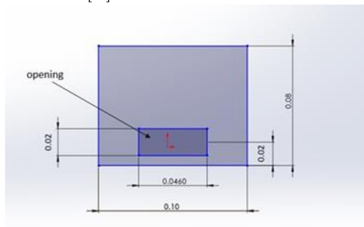
Fig 3.3: View of the model from inlet considered for validation as studied by Karava et al, (2011) [27]
