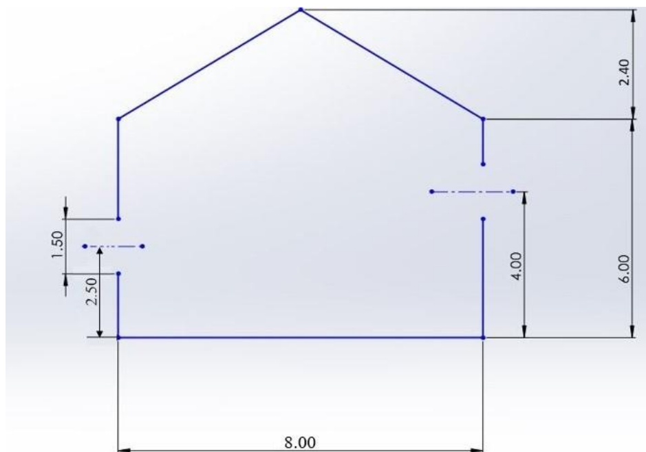
Fig 4.3: Cross Sectional view of Configuration B
