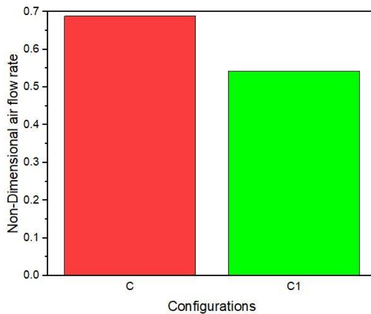
Fig 4.16: Comparison of non-dimensional air flow rate for configuration C and C1
