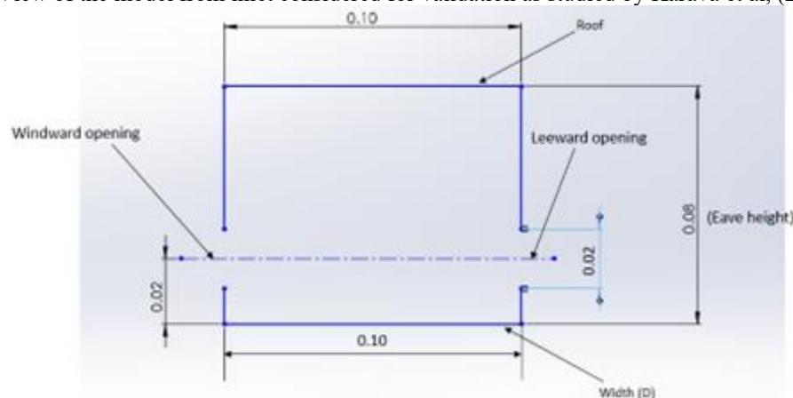
Fig 3.3: View of the model from inlet considered for validation as studied by Karava et al, (2011) [27]
