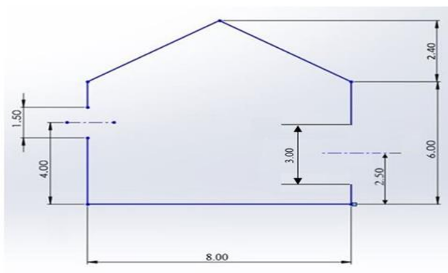
Fig 4.2a: Cross Sectional view of Configuration A1
