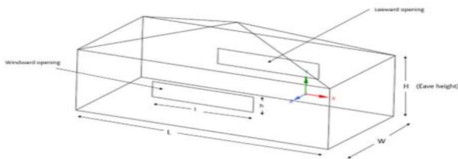
Fig 3.1: Three-dimensional view of the Pyramidal building
