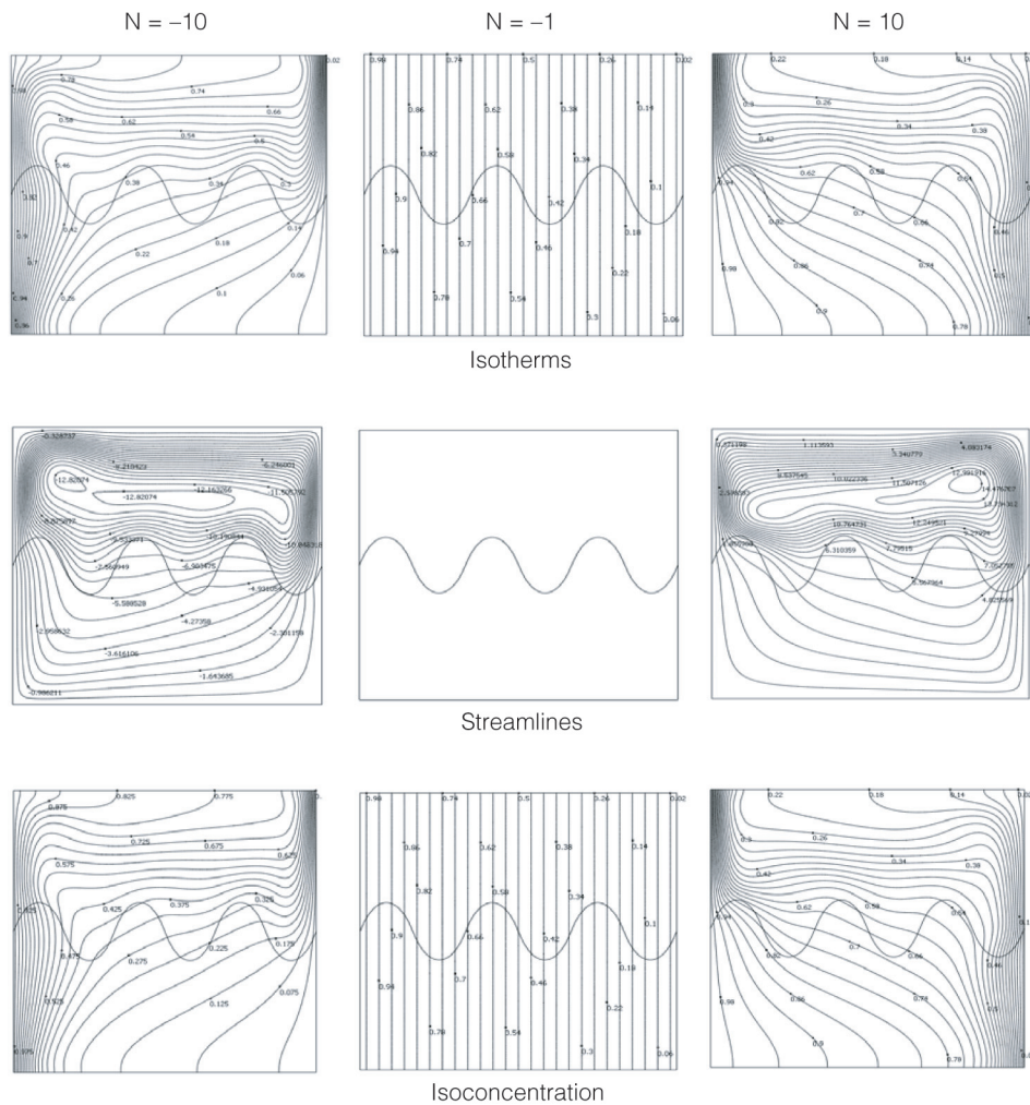
Figure 8 Isotherms Streamlines and Isoconcentration for Ra = 10^5 ; Da = 10^{-4} ; Le = 0, 84 ; n = 3 ; Pr = 0,71 , \varepsilon = 0,5 , A = 0,1 and N = 10; -1, -10 .
