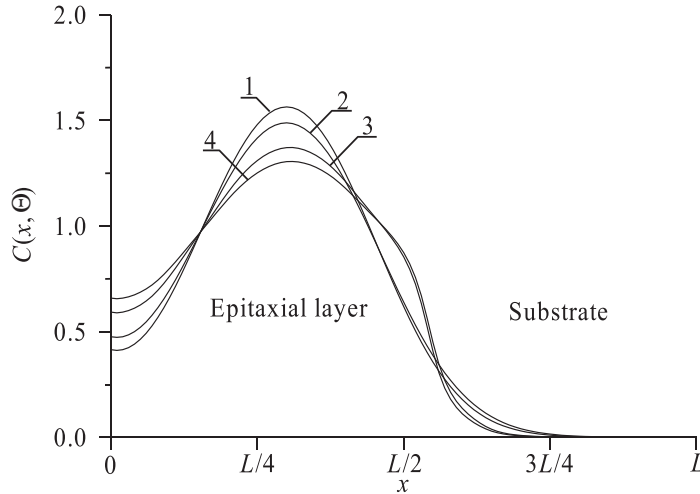
Figure 3: Distributions of concentration of implanted dopant in heterostructure from Fig. 1 in direction, which is perpendicular to interface between epitaxial layer substrate. Curves 1 and 3 corresponds to annealing time \Theta = 0.0048(L_x^2 + L_y^2 + L_z^2)/D_0 . Curves 2 and 4 corresponds to annealing time \Theta = 0.0057(L_x^2 + L_y^2 + L_z^2)/D_0 . Curves 1 and 2 corresponds to homogenous sample. Curves 3 and 4 corresponds to heterostructure under condition, when value of dopant diffusion coefficient in epitaxial layer is larger, than value of dopant diffusion coefficient in substrate
